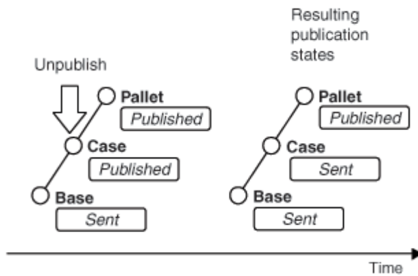
Figure 143: Revocation of publication of a part of the hierarchy
