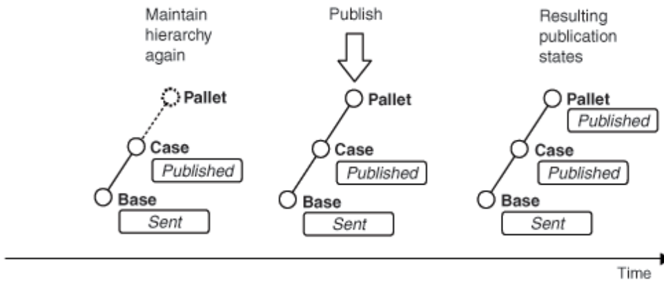
Figure 142: Enhancement of subsequent of the simple hierarchy
