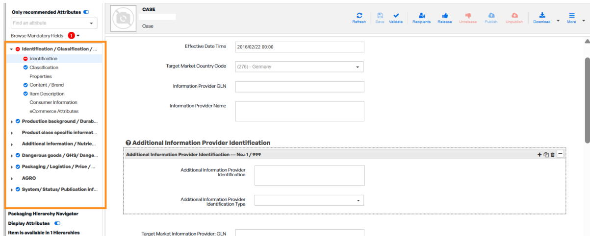
Figure 59: Structure of the editor – edit form with function bar
