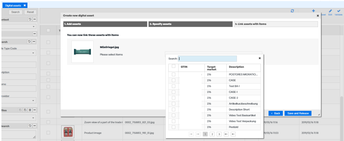
Figure 180: Link Assets to an item
