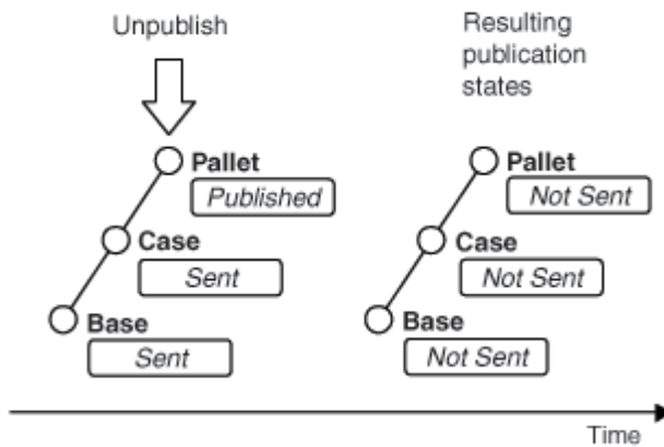
Figure 144: Revocation of publication of the entire hierarchy
