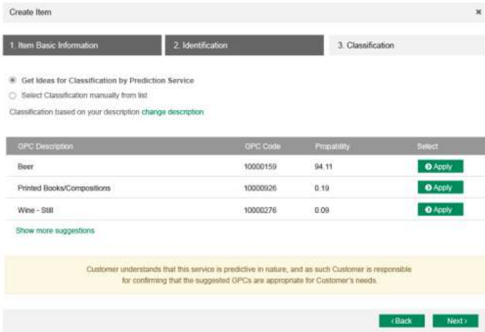
Figure 17: Creation Wizard, Classification
