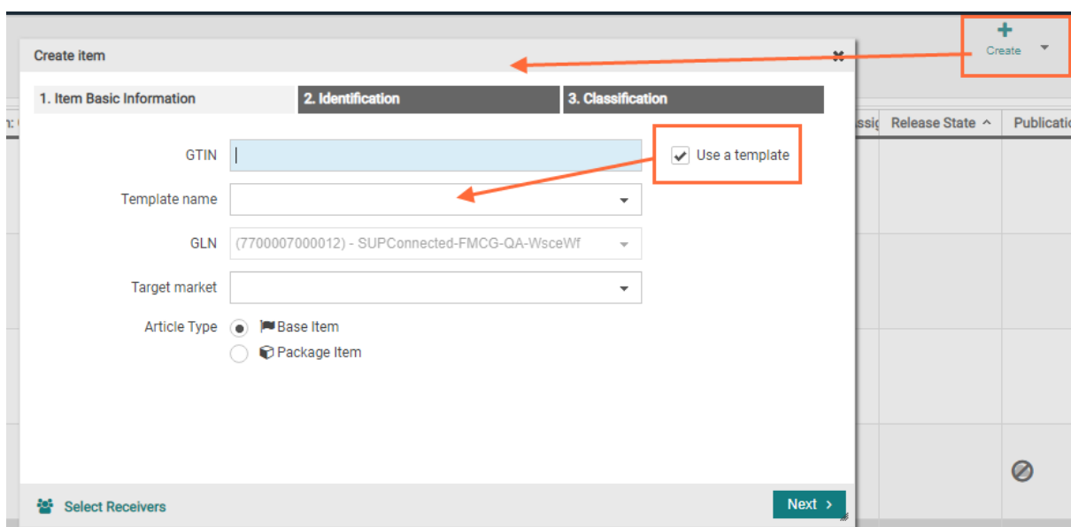
Figure 124: Create item using a template
