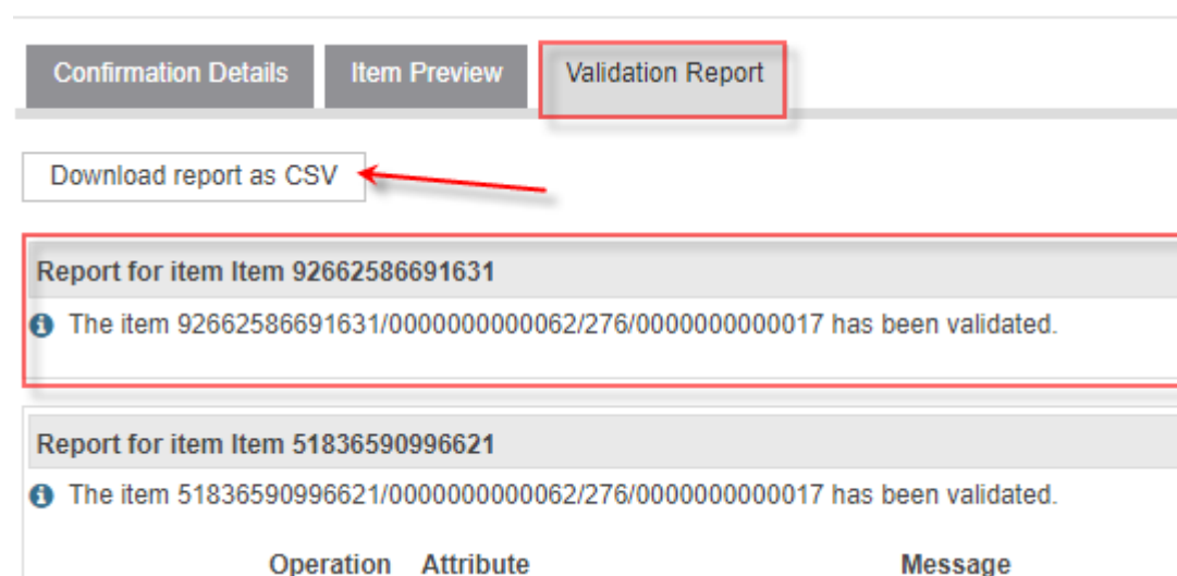
Figure 81: Validation Report
