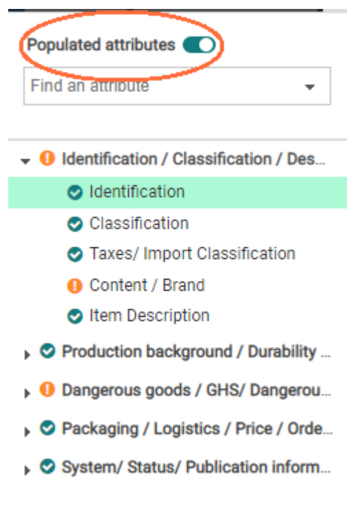
Figure 30: Populated attributes-switch
