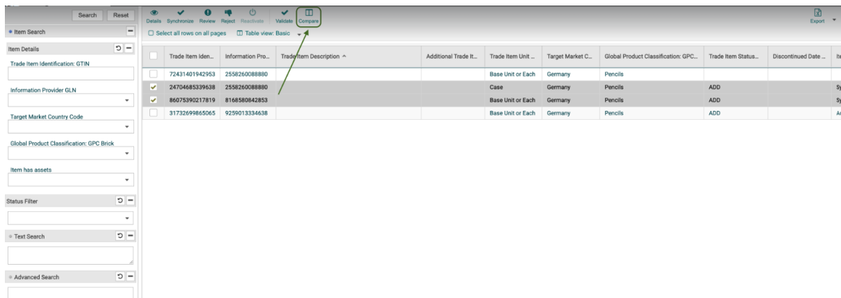
Figure 65: Compare GTINs
